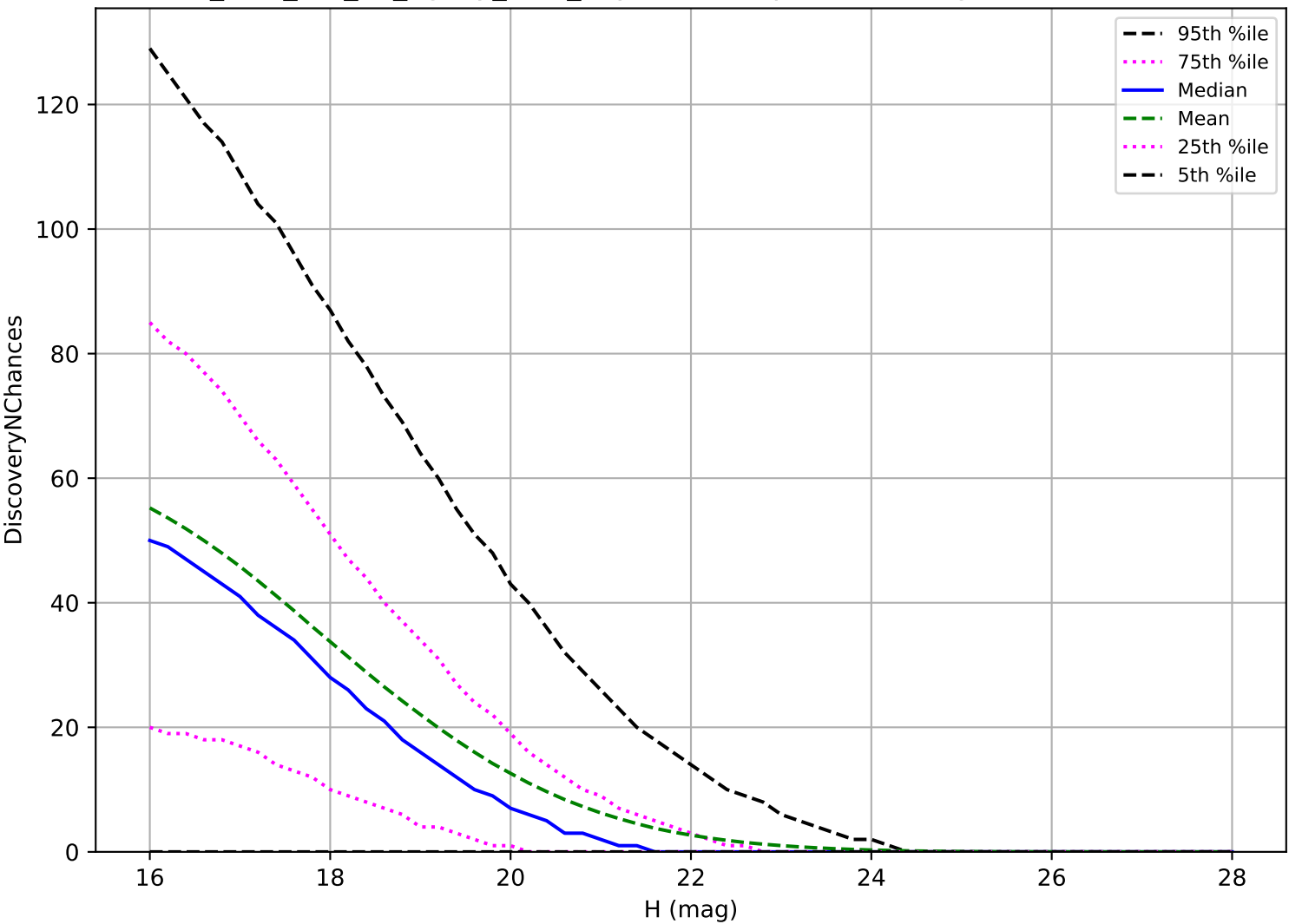
too_elab_r32_d2_ugrizy_v3.4_10yrs: NEO 3 pairs in 15 nights detection loss
