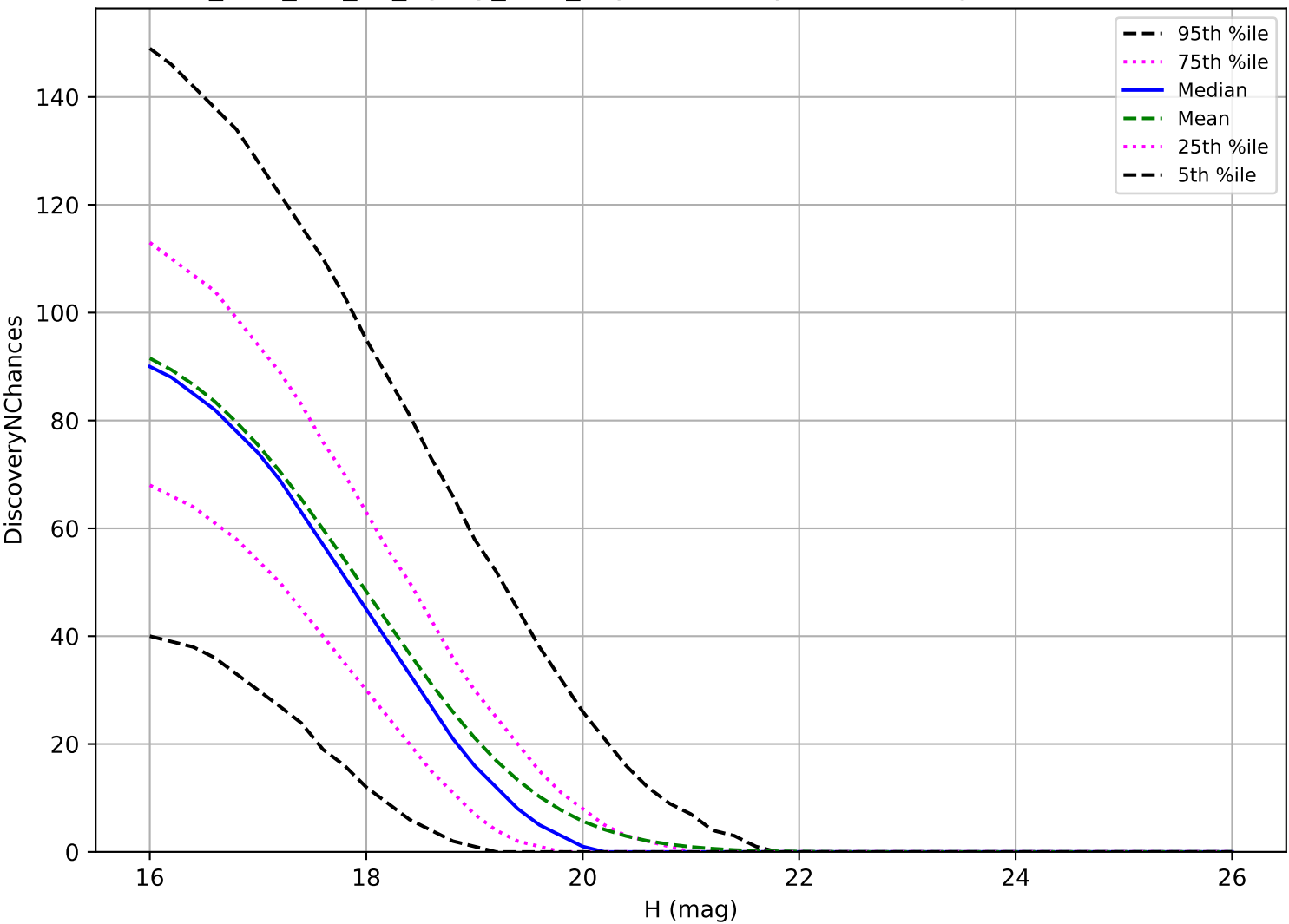
too_elab_r32_d2_ugrizy_v3.4_10yrs: MBA 3 pairs in 15 nights detection loss
