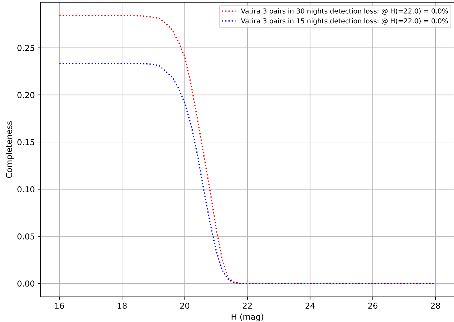
too_elab_r32_d2_ugrizy_v3.4_10yrs: DifferentialCompleteness
