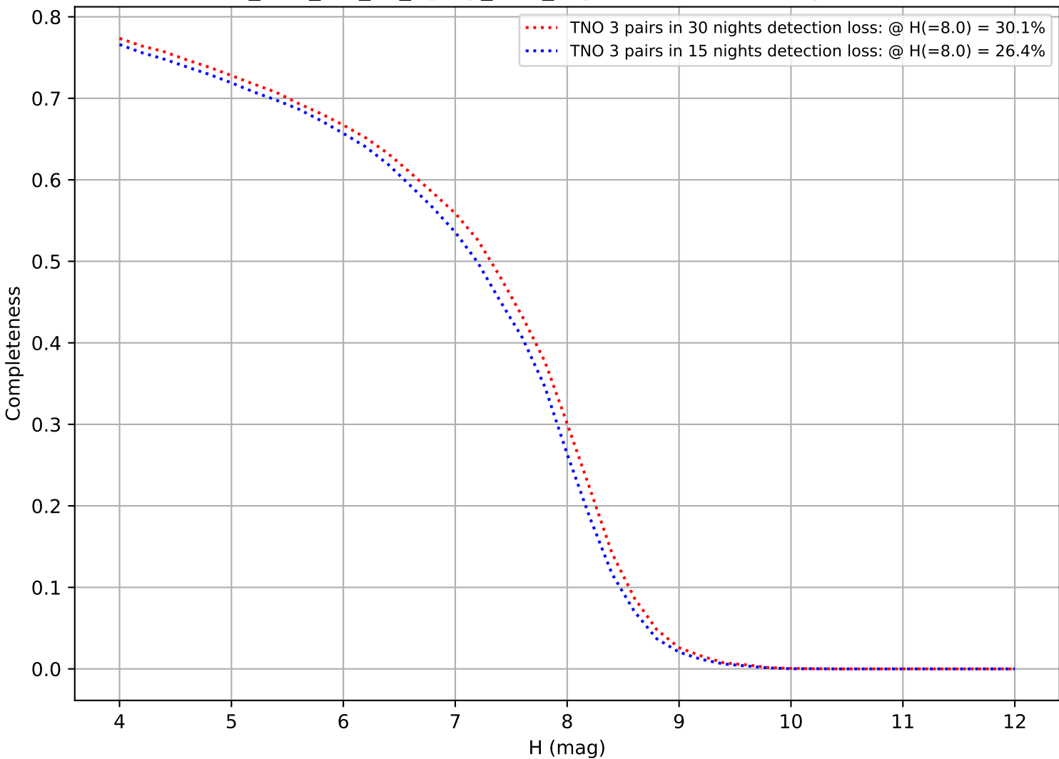
too_elab_r32_d2_ugrizy_v3.4_10yrs: DifferentialCompleteness
