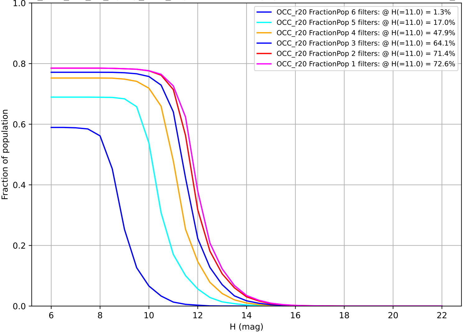
too_elab_r32_d2_ugrizy_v3.4_10yrs: Fraction of population with colors in X filters OCC_r20
