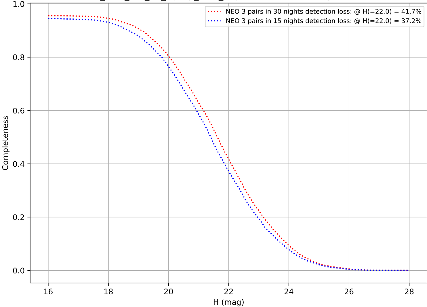
too_elab_r32_d2_ugrizy_v3.4_10yrs: DifferentialCompleteness
