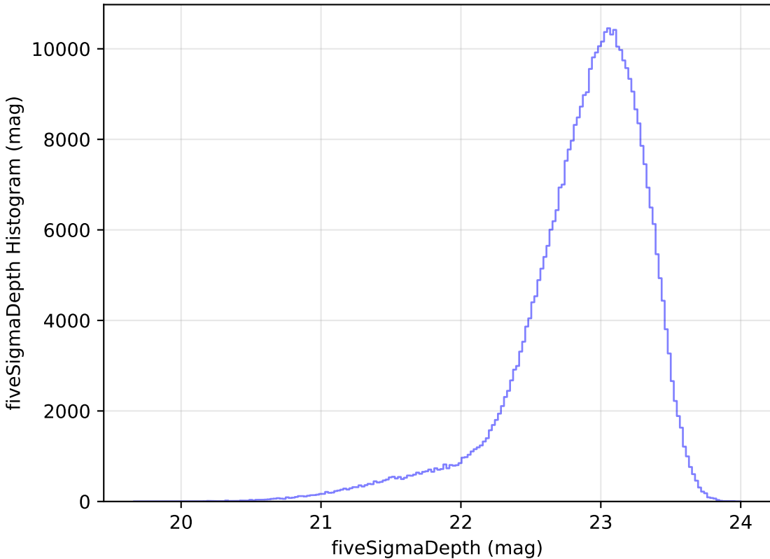
too_elab_r32_d2_ugrizy_v3.4_10yrs z: fiveSigmaDepth Histogram
