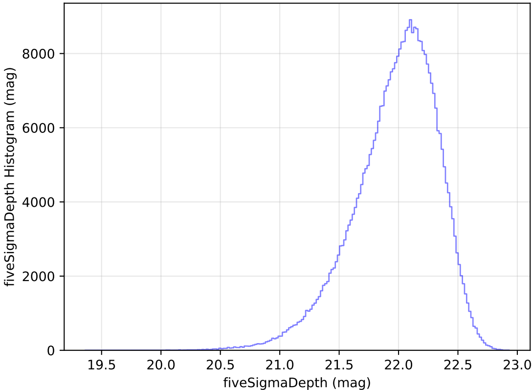
too_elab_r32_d2_ugrizy_v3.4_10yrs y: fiveSigmaDepth Histogram
