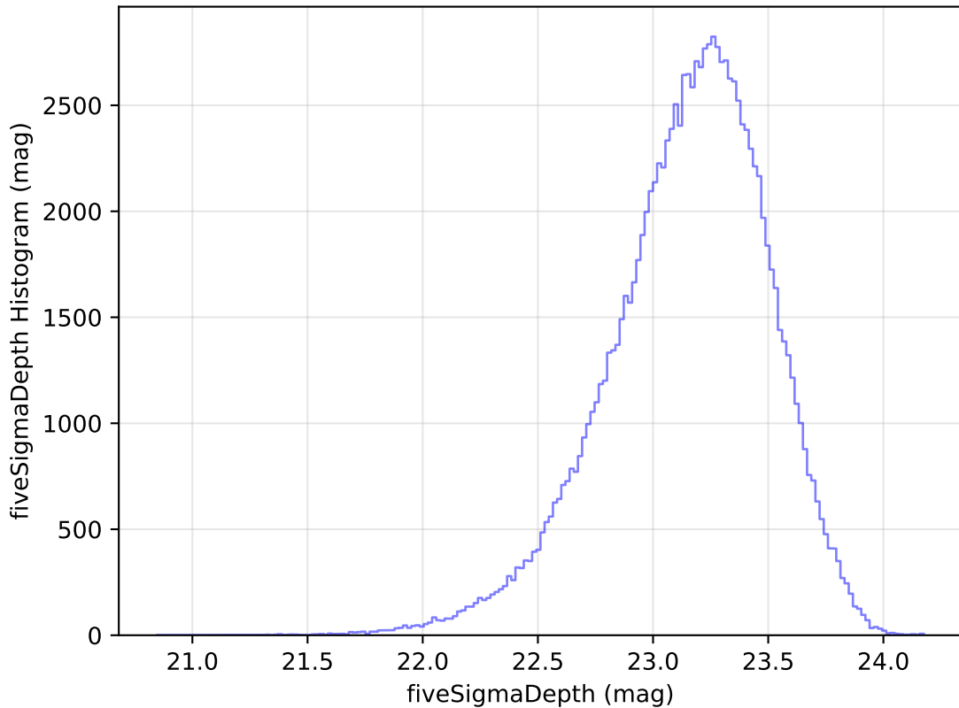
too_elab_r32_d2_ugrizy_v3.4_10yrs u: fiveSigmaDepth Histogram
