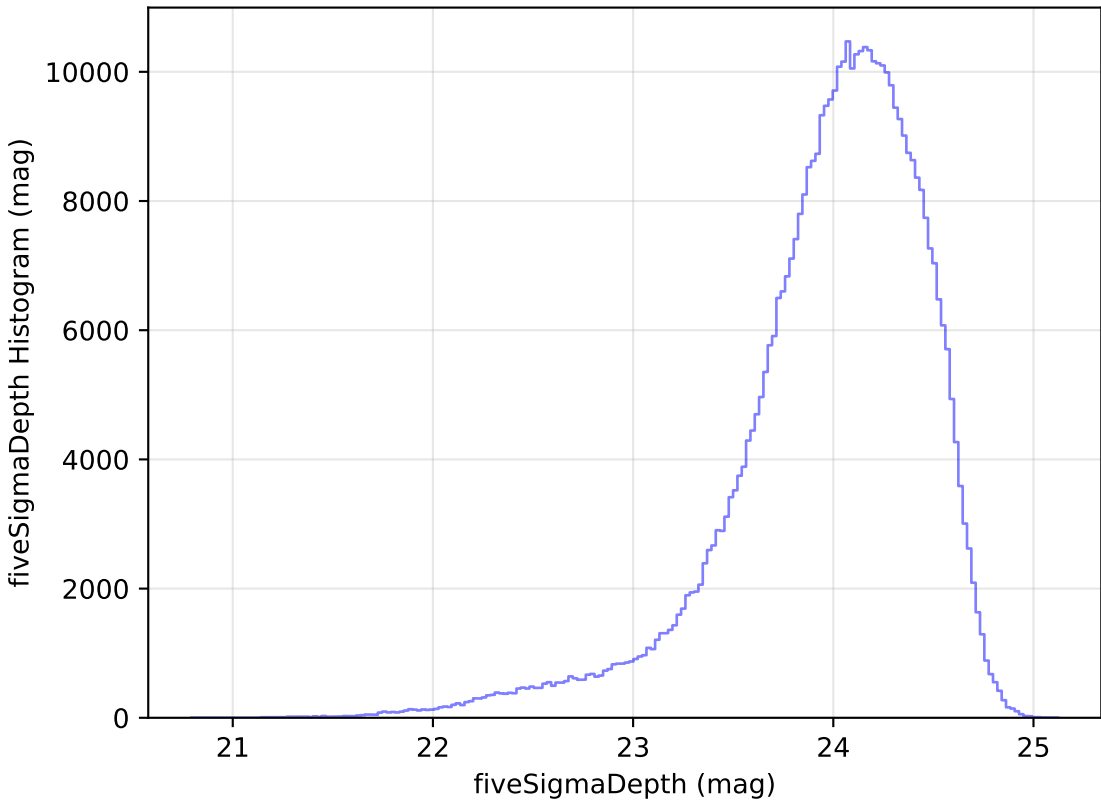
too_elab_r32_d2_ugrizy_v3.4_10yrs r: fiveSigmaDepth Histogram
