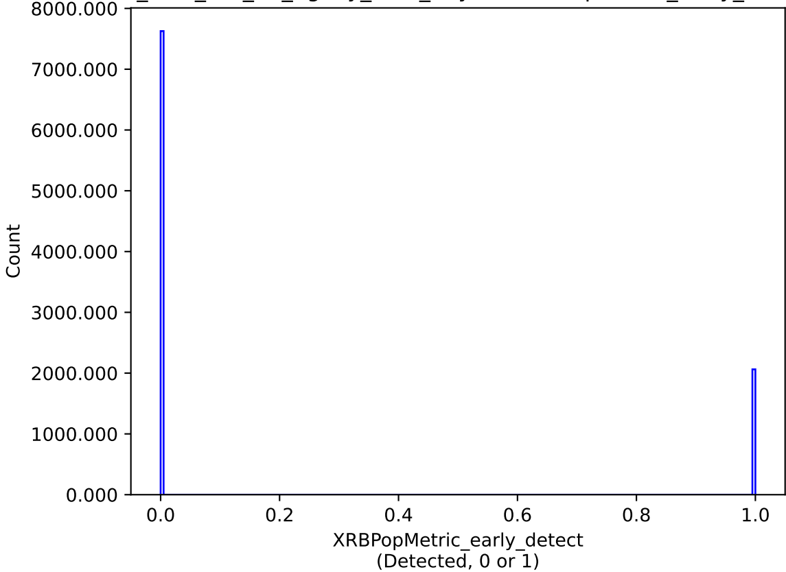
too_elab_r32_d2_ugrizy_v3.4_10yrs : XRBPopMetric_early_detect
