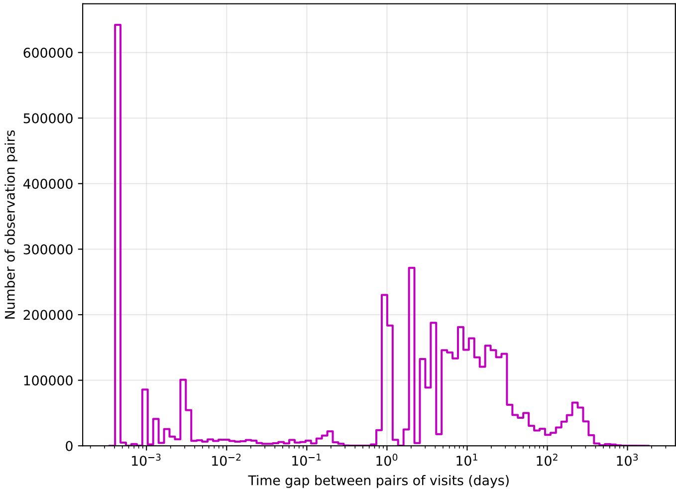
too_elab_r32_d2_ugrizy_v3.4_10yrs z band: Tgaps observationStartMJD
