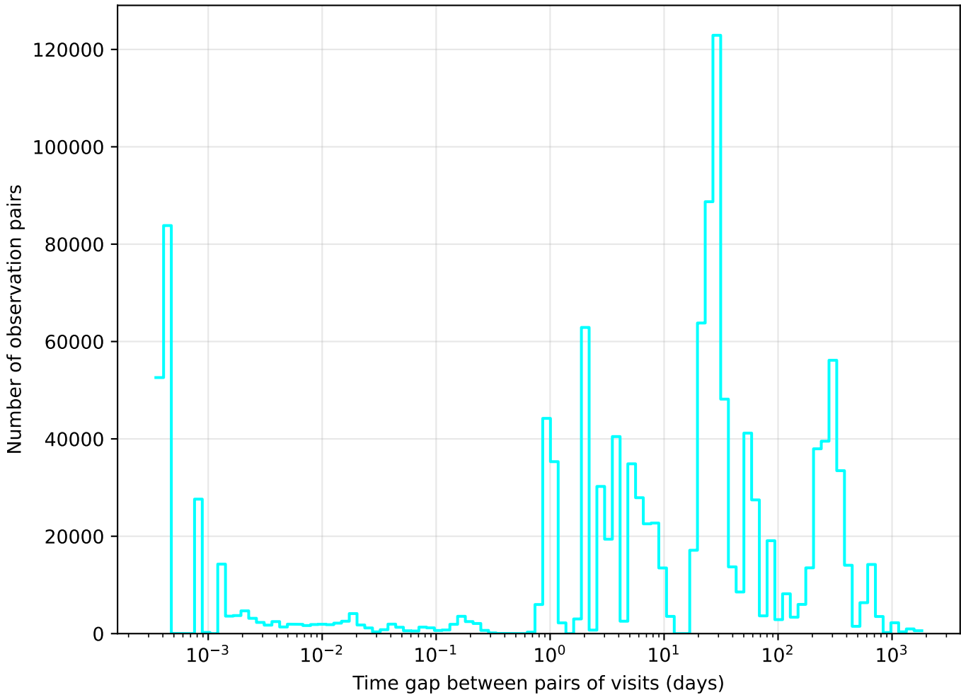
too_elab_r32_d2_ugrizy_v3.4_10yrs u band: Tgaps observationStartMJD
