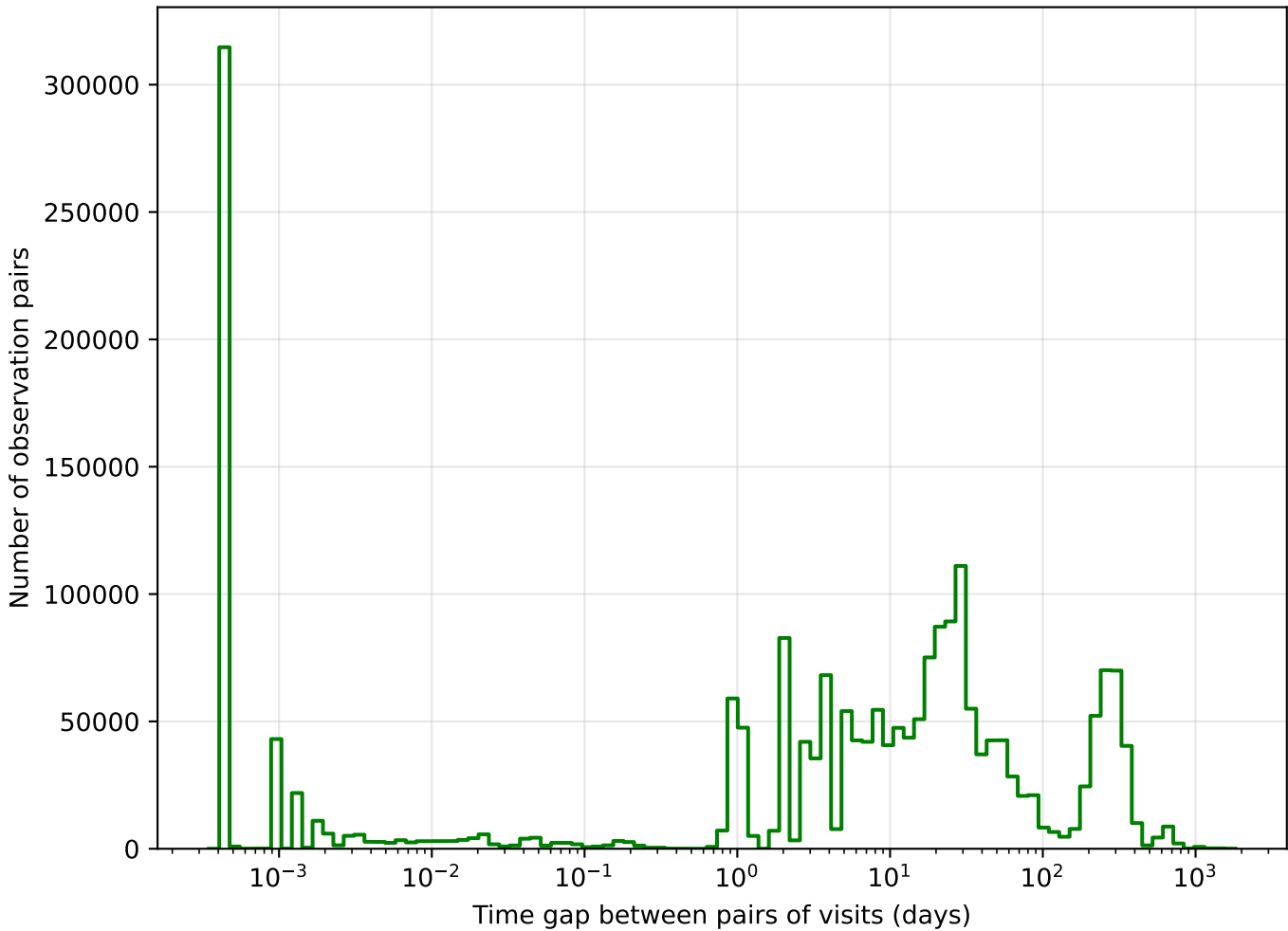
too_elab_r32_d2_ugrizy_v3.4_10yrs g band: Tgaps observationStartMJD
