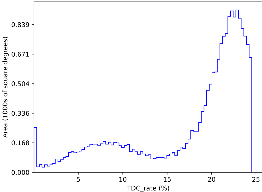
too_elab_r32_d2_ugrizy_v3.4_10yrs : TDC_rate
