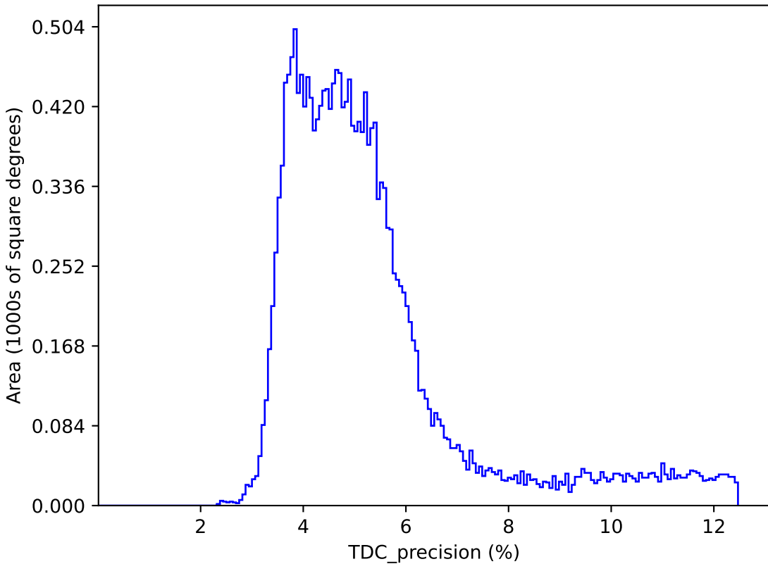
too_elab_r32_d2_ugrizy_v3.4_10yrs : TDC_precision
