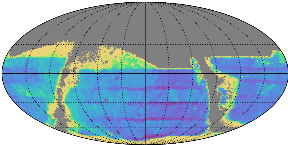
too_elab_r32_d2_ugrizy_v3.4_10yrs : TDC_accuracy
