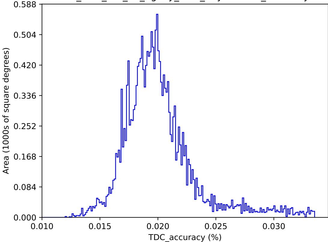
too_elab_r32_d2_ugrizy_v3.4_10yrs : TDC_accuracy
