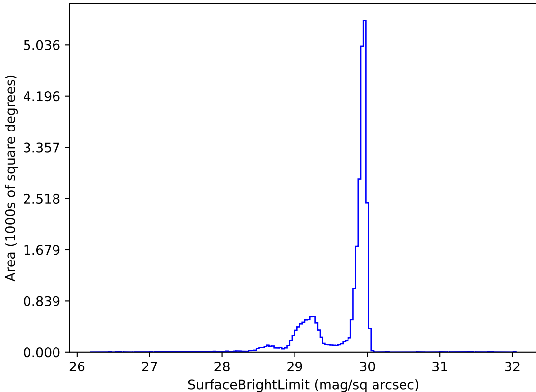
too_elab_r32_d2_ugrizy_v3.4_10yrs i: SurfaceBrightLimit
