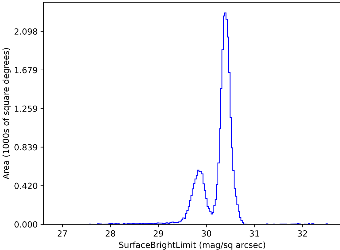
too_elab_r32_d2_ugrizy_v3.4_10yrs g: SurfaceBrightLimit
