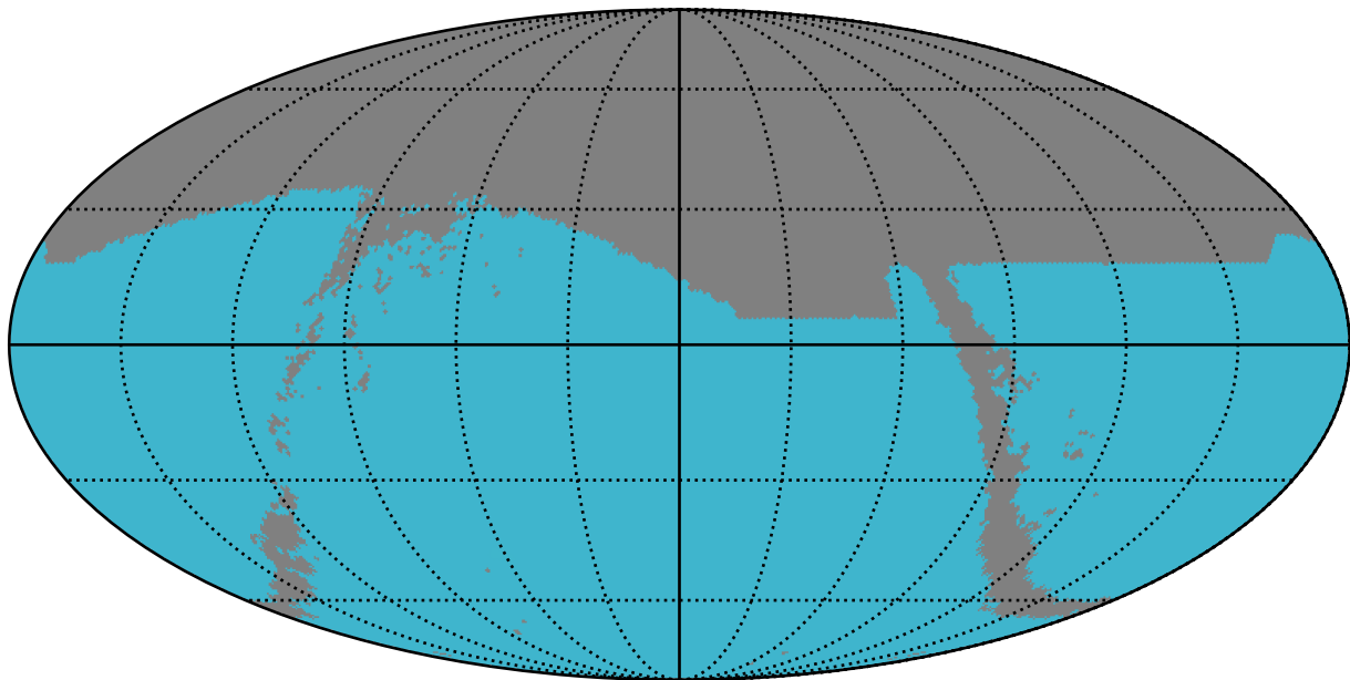
too_elab_r32_d2_ugrizy_v3.4_10yrs : SNSLMetric
