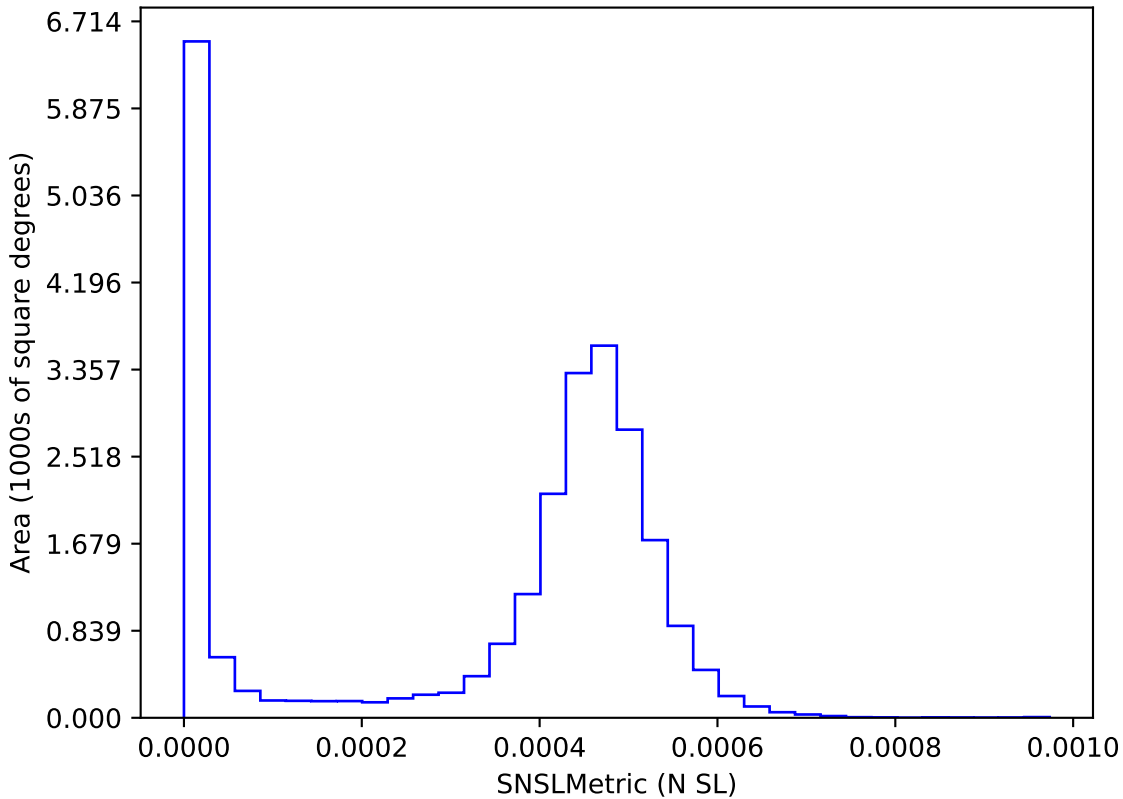
too_elab_r32_d2_ugrizy_v3.4_10yrs : SNSLMetric
