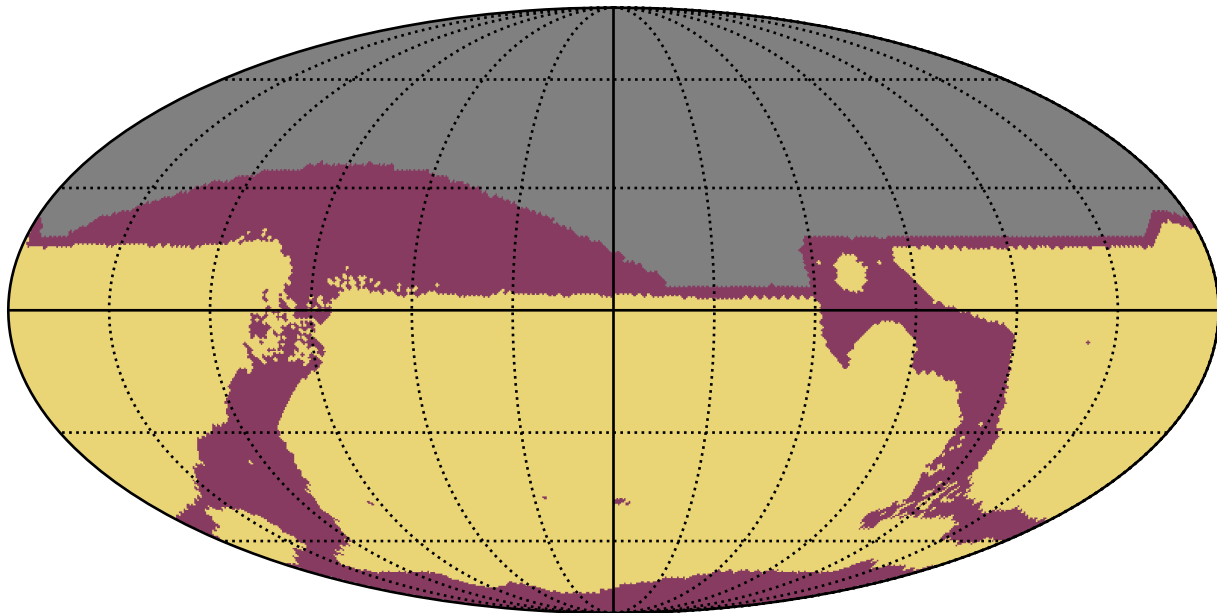
too_elab_r32_d2_ugrizy_v3.4_10yrs : RapidRevisits
