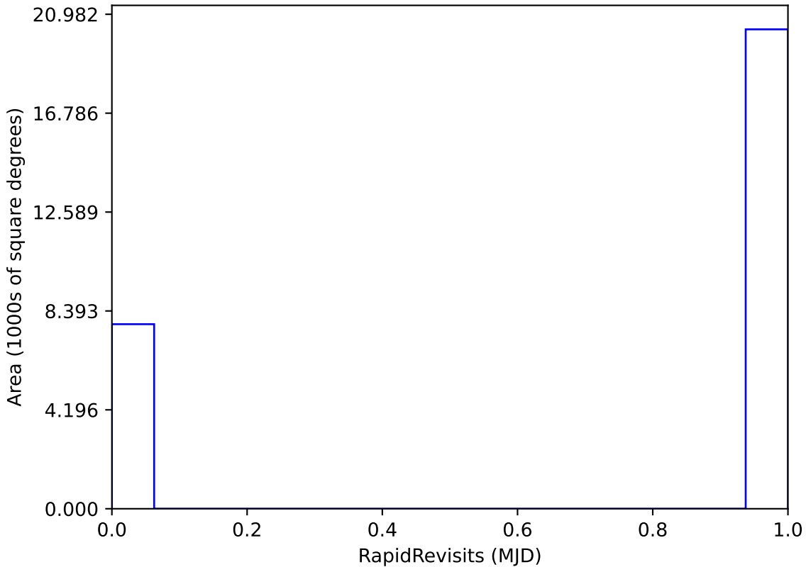
too_elab_r32_d2_ugrizy_v3.4_10yrs : RapidRevisits
