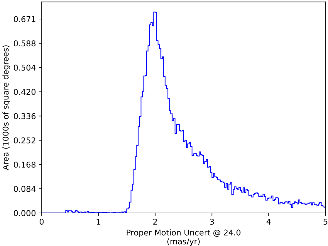
too_elab_r32_d2_ugrizy_v3.4_10yrs : Proper Motion Uncert @ 24.0
