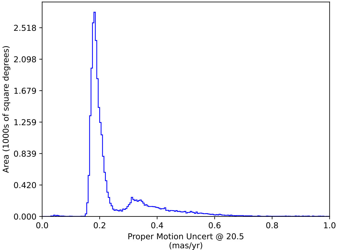
too_elab_r32_d2_ugrizy_v3.4_10yrs : Proper Motion Uncert @ 20.5
