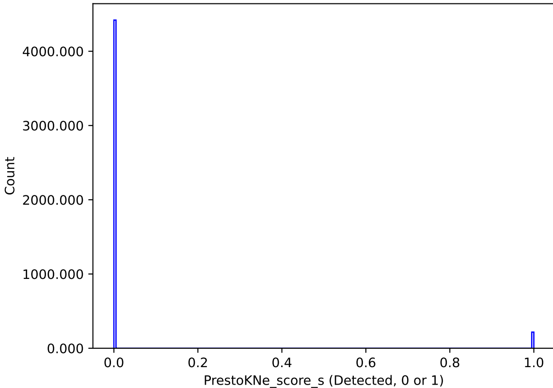
too_elab_r32_d2_ugrizy_v3.4_10yrs : PrestoKNe_score_s
