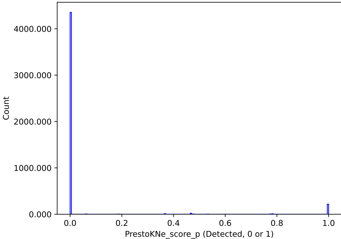
too_elab_r32_d2_ugrizy_v3.4_10yrs : PrestoKNe_score_p
