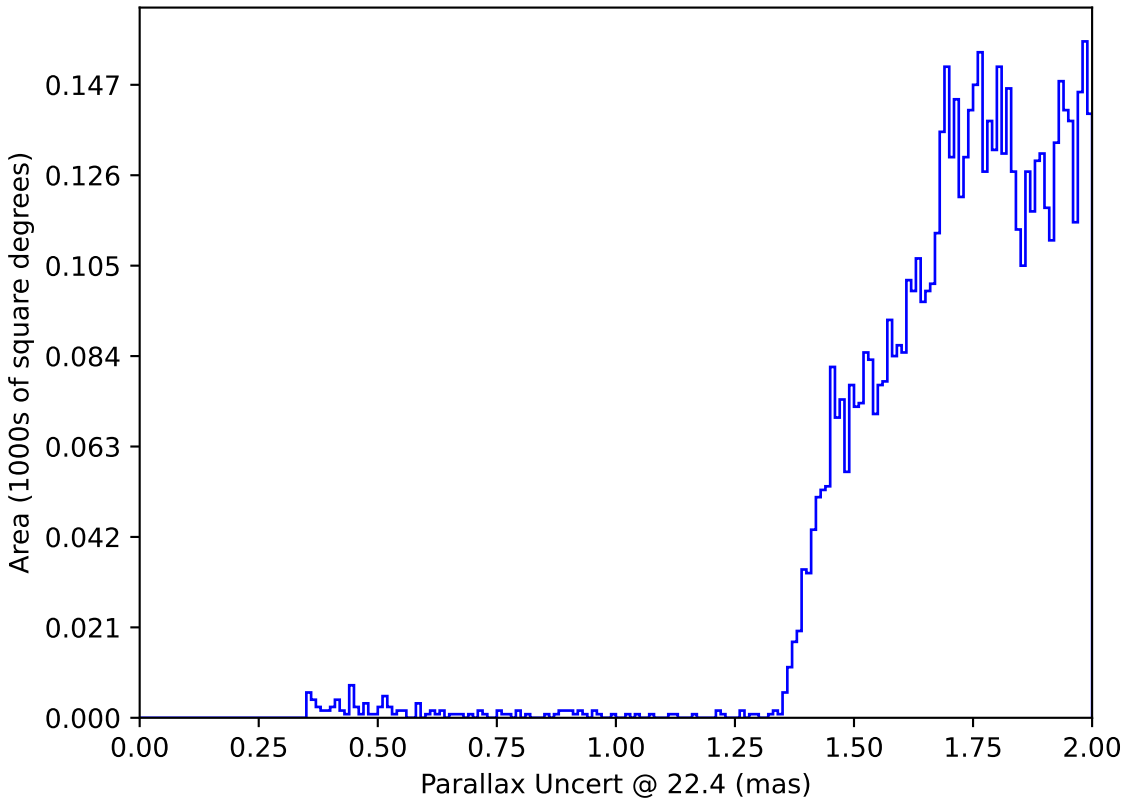
too_elab_r32_d2_ugrizy_v3.4_10yrs : Parallax Uncert @ 22.4
