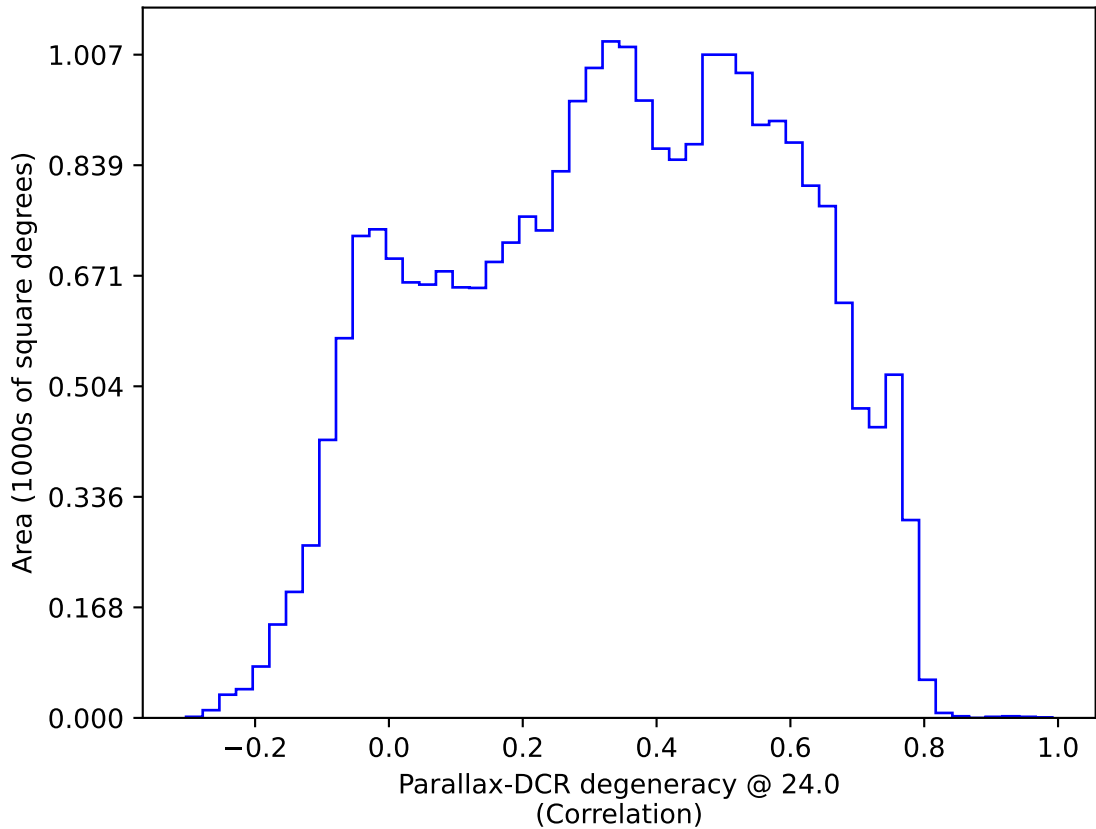
too_elab_r32_d2_ugrizy_v3.4_10yrs : Parallax-DCR degeneracy @ 24.0
