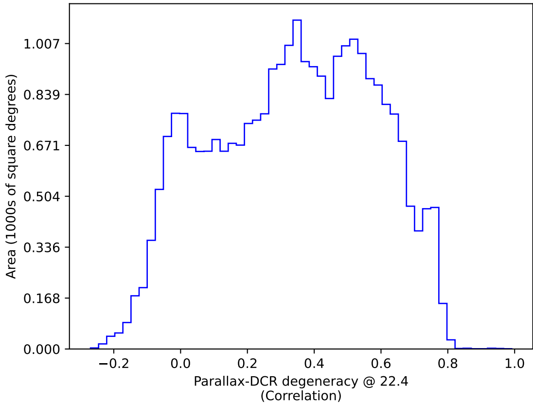
too_elab_r32_d2_ugrizy_v3.4_10yrs : Parallax-DCR degeneracy @ 22.4
