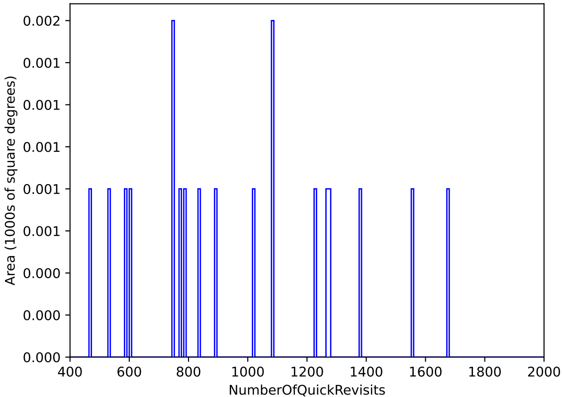
too_elab_r32_d2_ugrizy_v3.4_10yrs : NumberOfQuickRevisits
