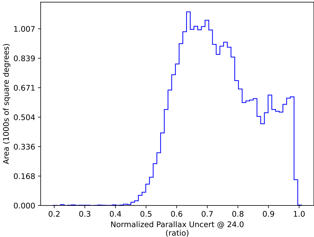
too_elab_r32_d2_ugrizy_v3.4_10yrs : Normalized Parallax Uncert @ 24.0
