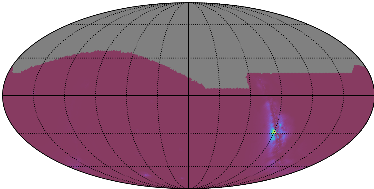
too_elab_r32_d2_ugrizy_v3.4_10yrs : NlcPoints
