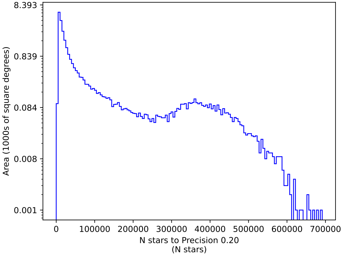
too_elab_r32_d2_ugrizy_v3.4_10yrs z: N stars to Precision 0.20
