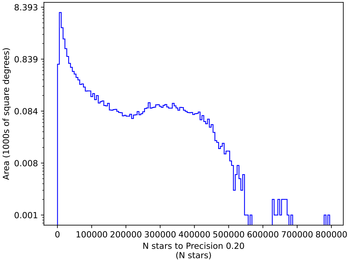
too_elab_r32_d2_ugrizy_v3.4_10yrs y: N stars to Precision 0.20
