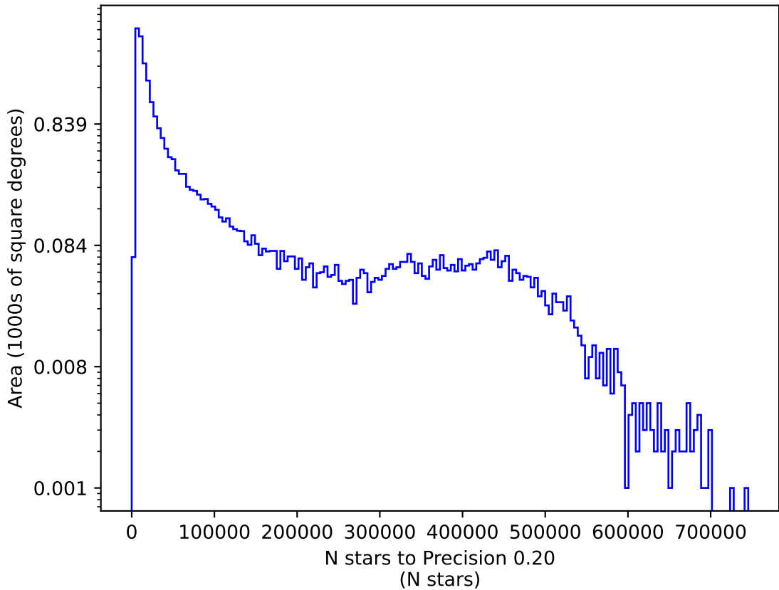
too_elab_r32_d2_ugrizy_v3.4_10yrs r: N stars to Precision 0.20
