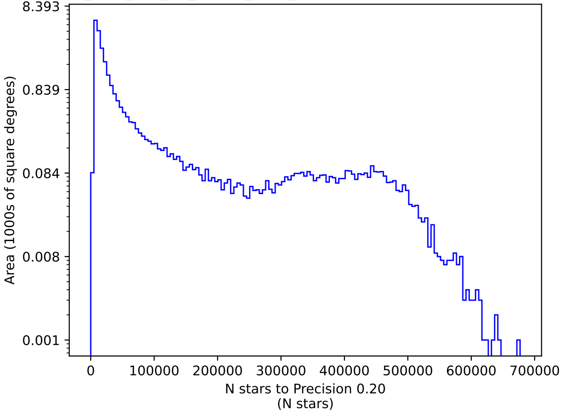
too_elab_r32_d2_ugrizy_v3.4_10yrs i: N stars to Precision 0.20
