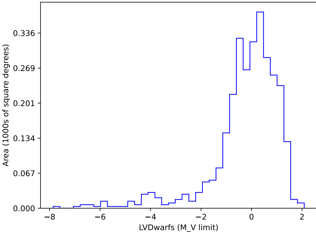
too_elab_r32_d2_ugrizy_v3.4_10yrs gi SCP: LVDwarfs
