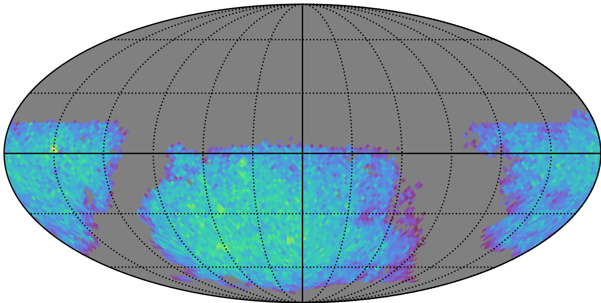
too_elab_r32_d2_ugrizy_v3.4_10yrs gi: LVDwarfs
