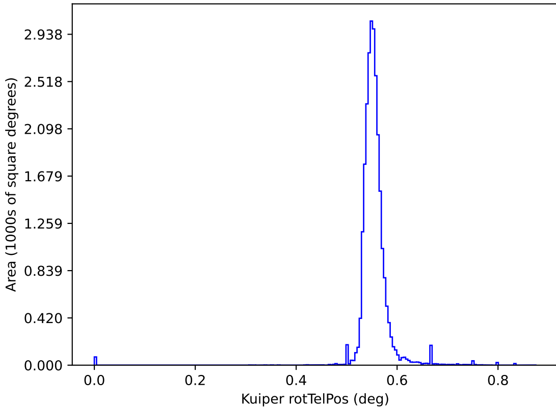
too_elab_r32_d2_ugrizy_v3.4_10yrs y: Kuiper rotTelPos
