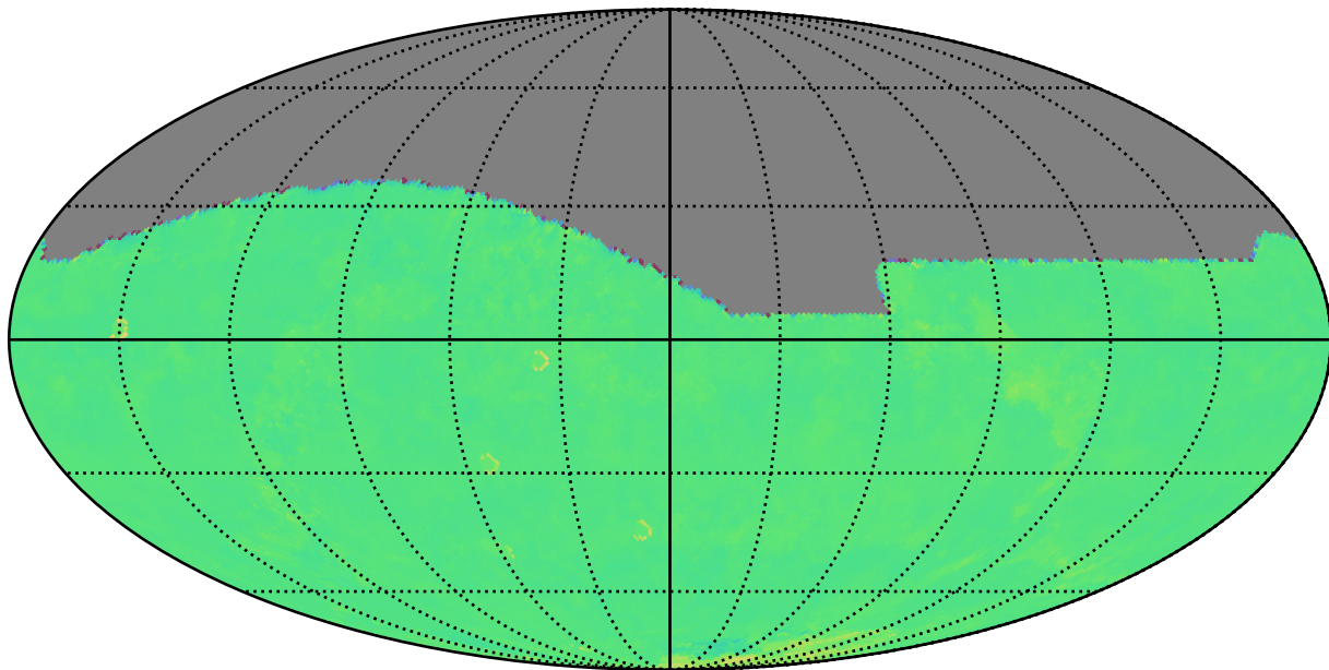
too_elab_r32_d2_ugrizy_v3.4_10yrs r: Kuiper rotTelPos
