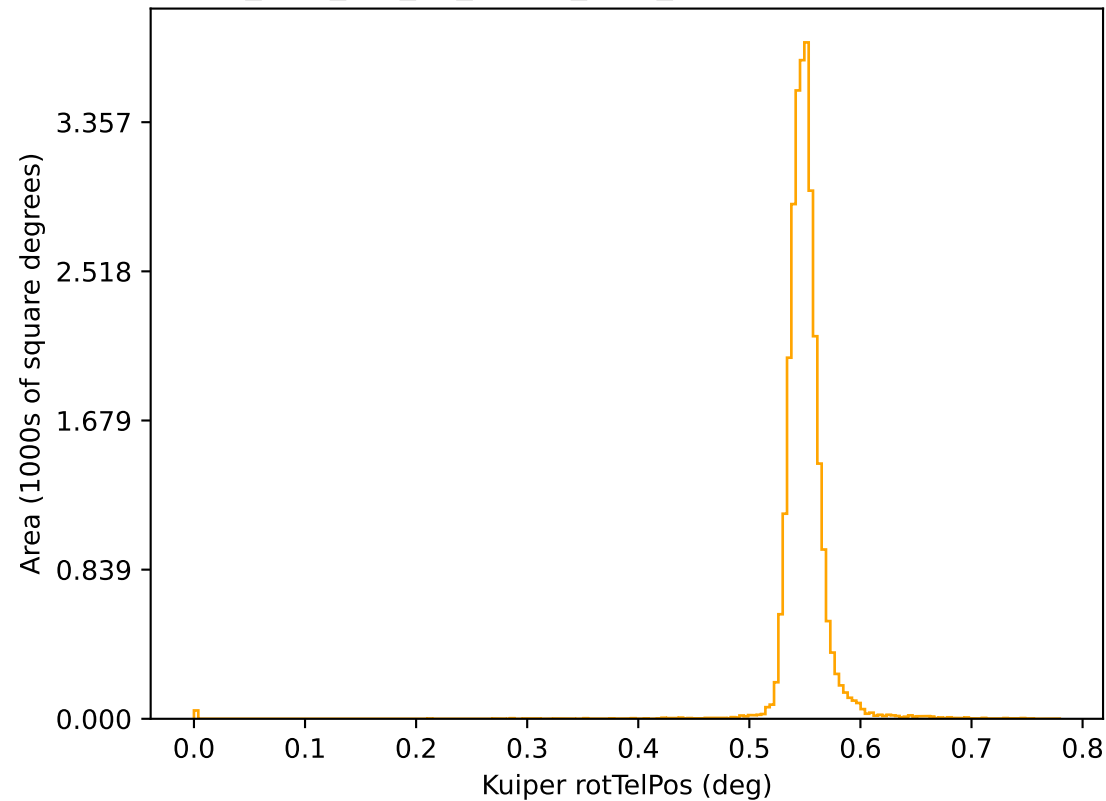
too_elab_r32_d2_ugrizy_v3.4_10yrs r: Kuiper rotTelPos
