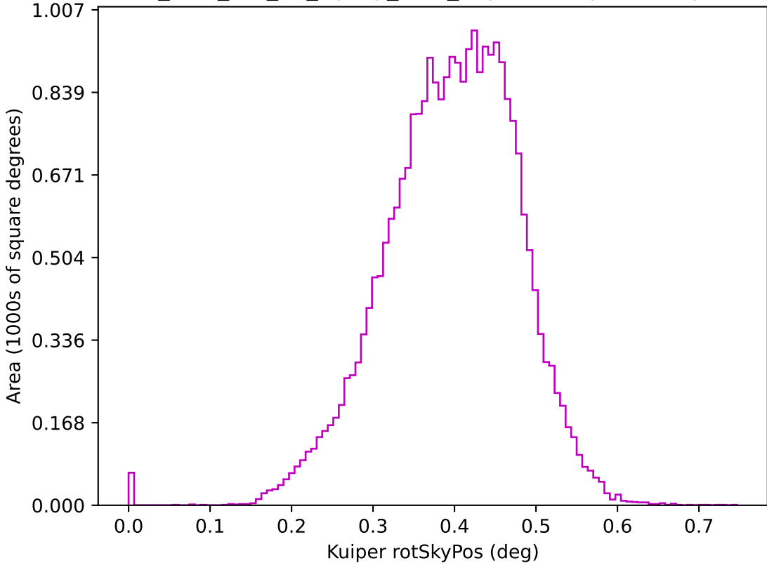
too_elab_r32_d2_ugrizy_v3.4_10yrs z: Kuiper rotSkyPos
