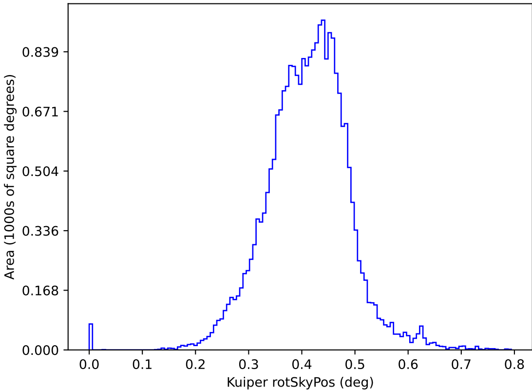
too_elab_r32_d2_ugrizy_v3.4_10yrs y: Kuiper rotSkyPos
