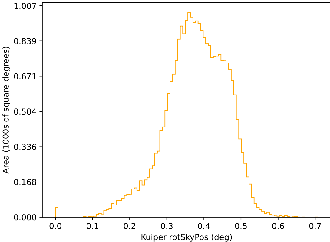
too_elab_r32_d2_ugrizy_v3.4_10yrs r: Kuiper rotSkyPos
