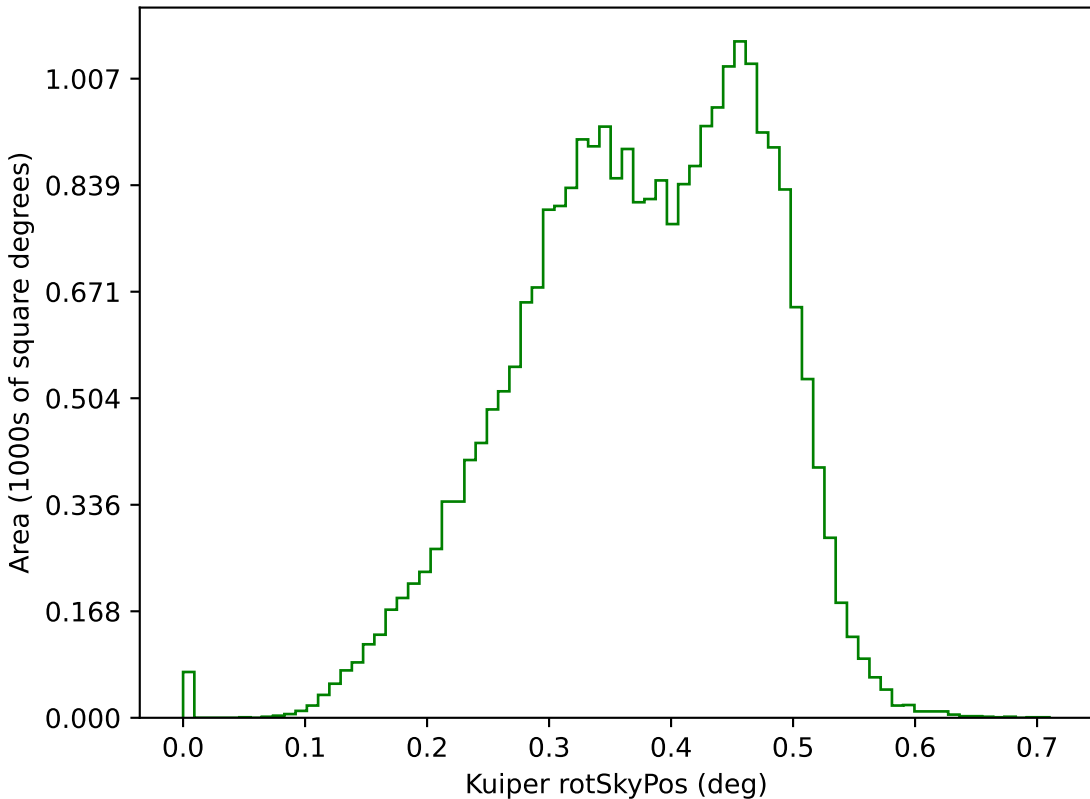
too_elab_r32_d2_ugrizy_v3.4_10yrs g: Kuiper rotSkyPos
