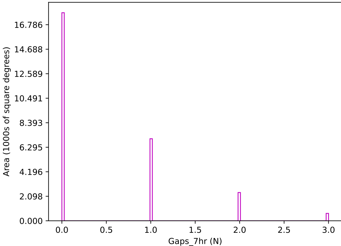
too_elab_r32_d2_ugrizy_v3.4_10yrs z band: Gaps_7hr
