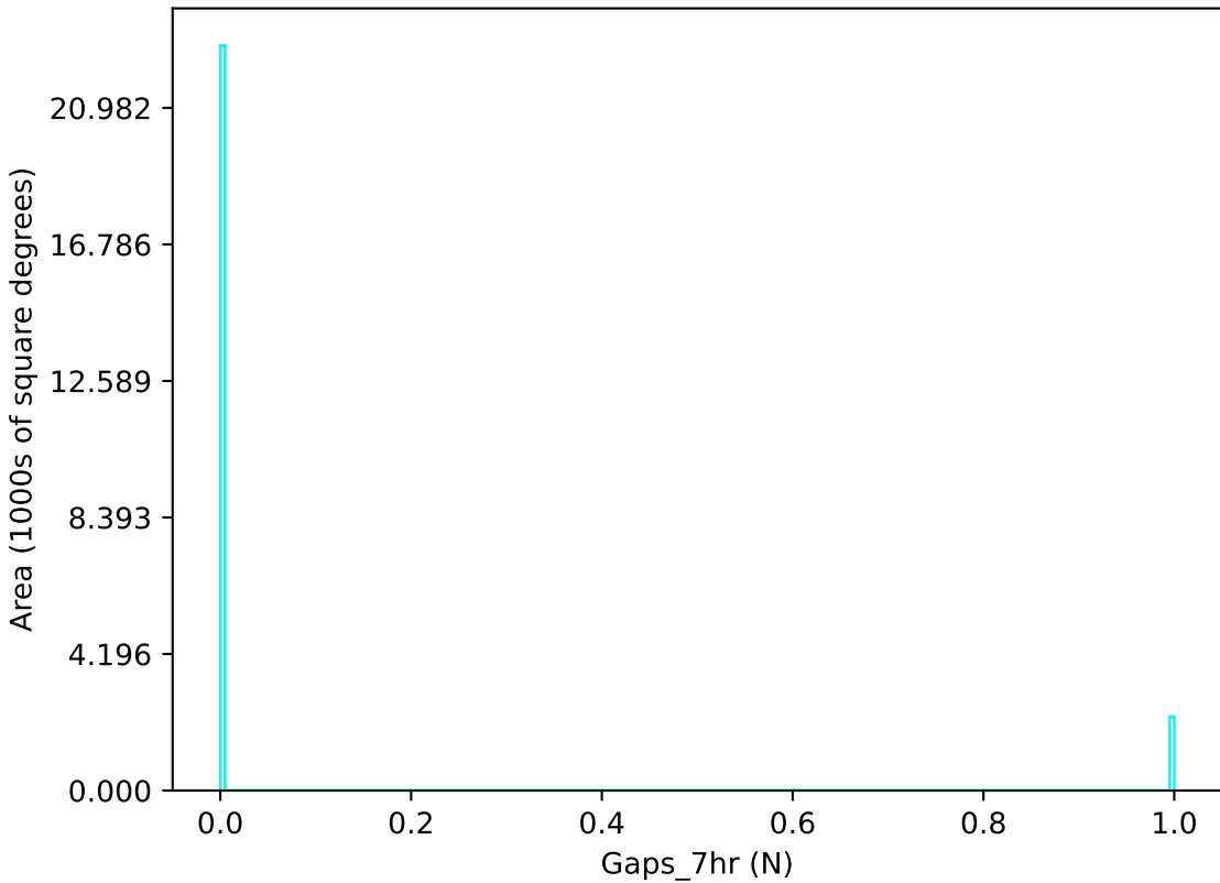
too_elab_r32_d2_ugrizy_v3.4_10yrs u band: Gaps_7hr
