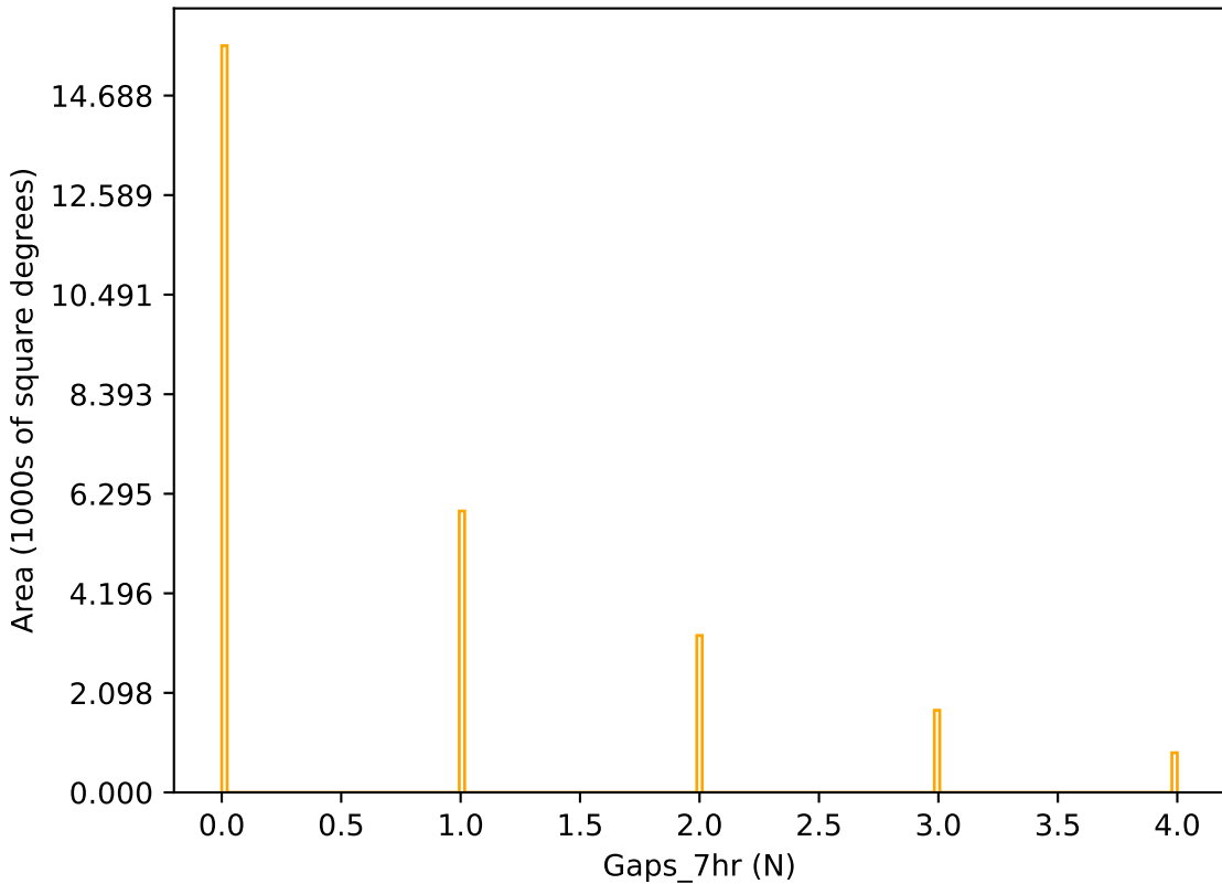
too_elab_r32_d2_ugrizy_v3.4_10yrs r band: Gaps_7hr
